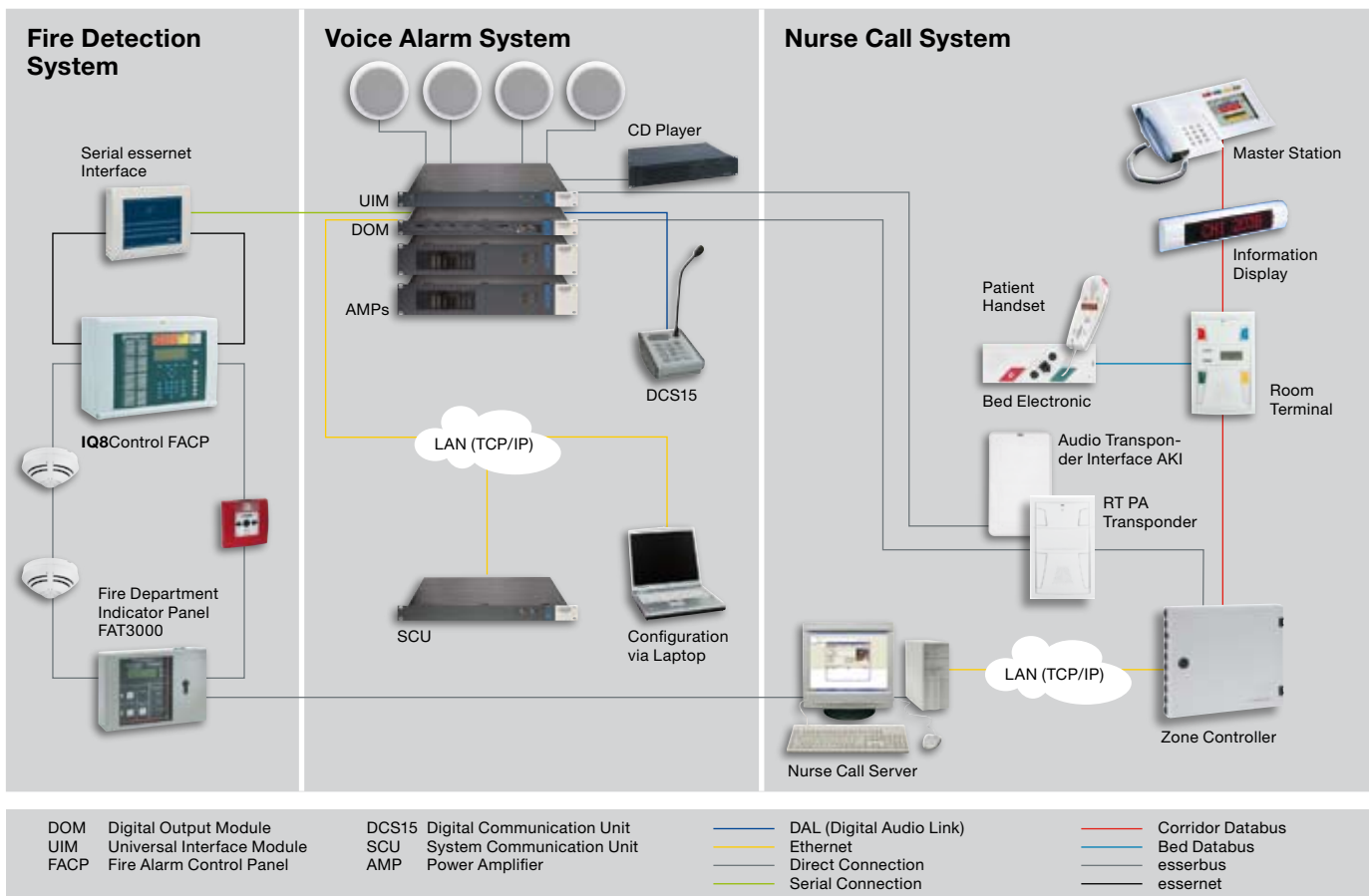
Basic circuiting for the connection of voice alarm components to fire detection technology and care communication
